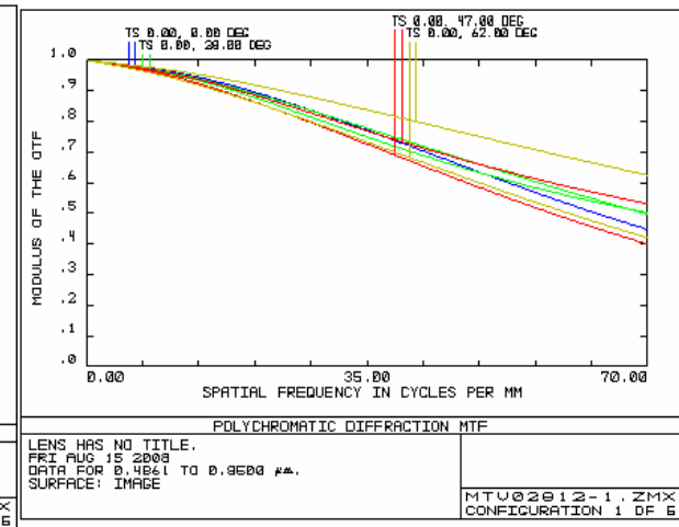
Short focus MTF
