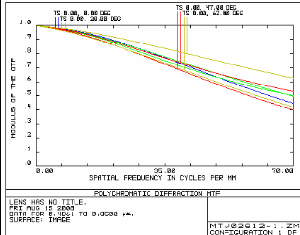
Long focus MTF
